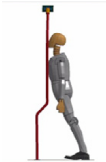
Pole with compliant mount at the top under emergency braking.
