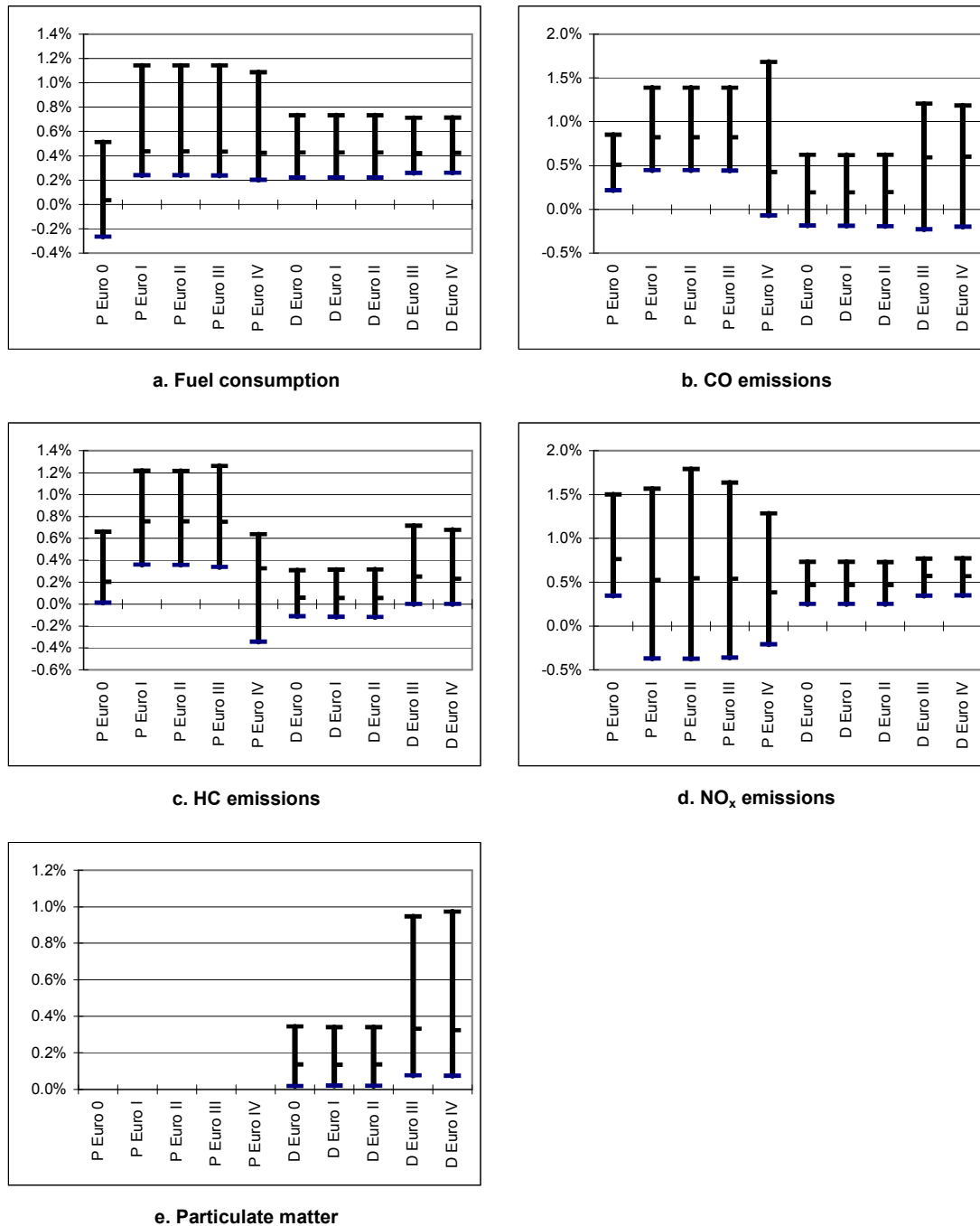
Figure 4: Range of relative changes in fuel consumption and emissions: +42W (showing 5th, 50th and 95th percentiles).
