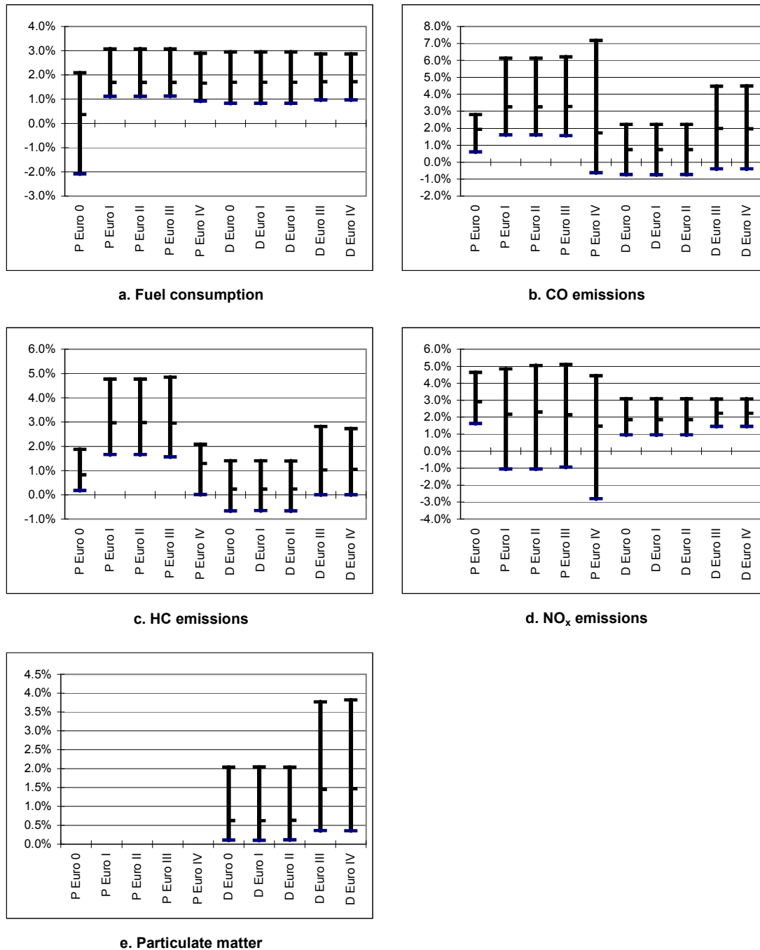
Figure 5: Range of relative changes in fuel consumption and emissions: +160W (showing 5th, 50th and 95th percentiles).
