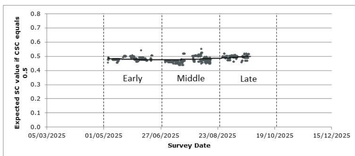
Figure 4.5: Expected SC if CSC equals 0.5 from SASS analysis
