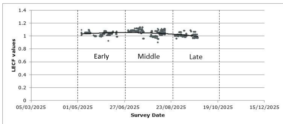
Figure 4.4: Distribution of LECF values by date from SASS analysis
